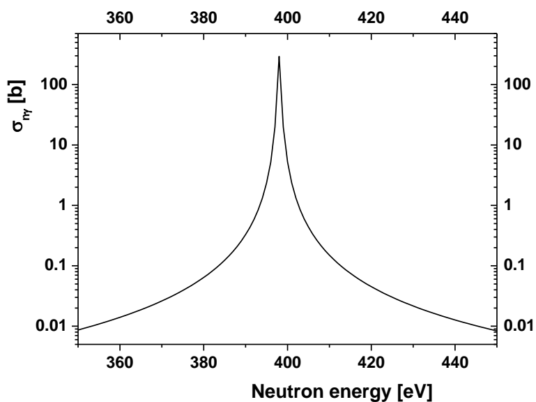
Figure 2: Cross sections calculated with formula (1) and parameters from (Brusegan, 2004); thin P-resonance with energy E_P = 398 eV in ^{35}\text{Cl}(n, \gamma)^{36}\text{Cl} reaction
