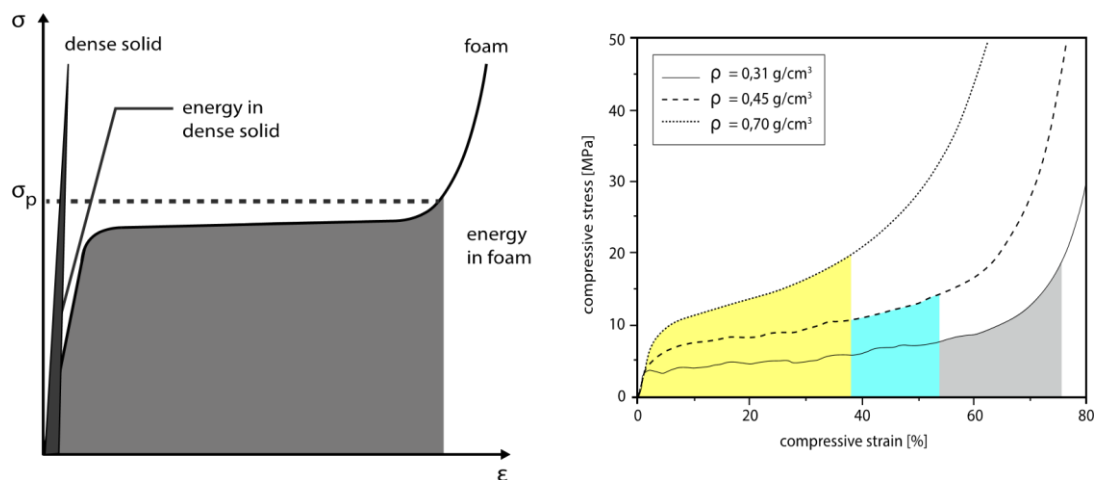
Figure 1: Left: Energy Absorption Comparison, Metallic Foam and Dense Material (Yu and Banhart, 1998). Right: Al-foams experimental test with three different density levels: 0.31 g/cm 3 , 0.45 g/cm 3 , and 0.70 g/cm 3 (Yu and Banhart, 1998)
