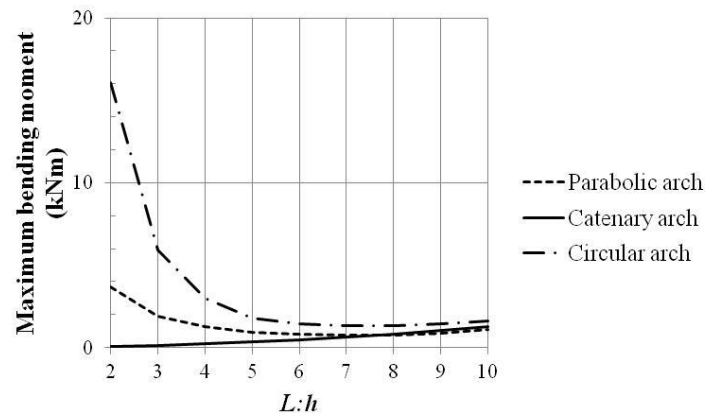
Figure 4. FE: The absolute value of maximum bending moment against L:h ratio; load case A3(SW only)
