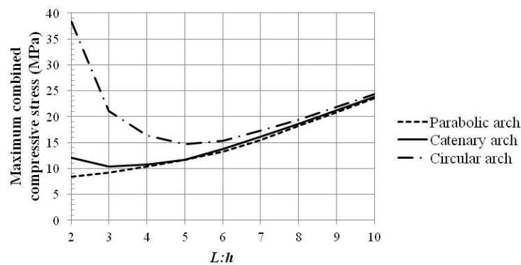
Figure 12. FE : The absolute value of the maximum combined stresses against L:h ratio using steel material for load case A1
