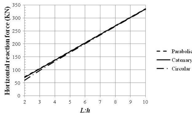
Figure 10. FE: The horizontal reaction force against L:h ratio; load case A1
